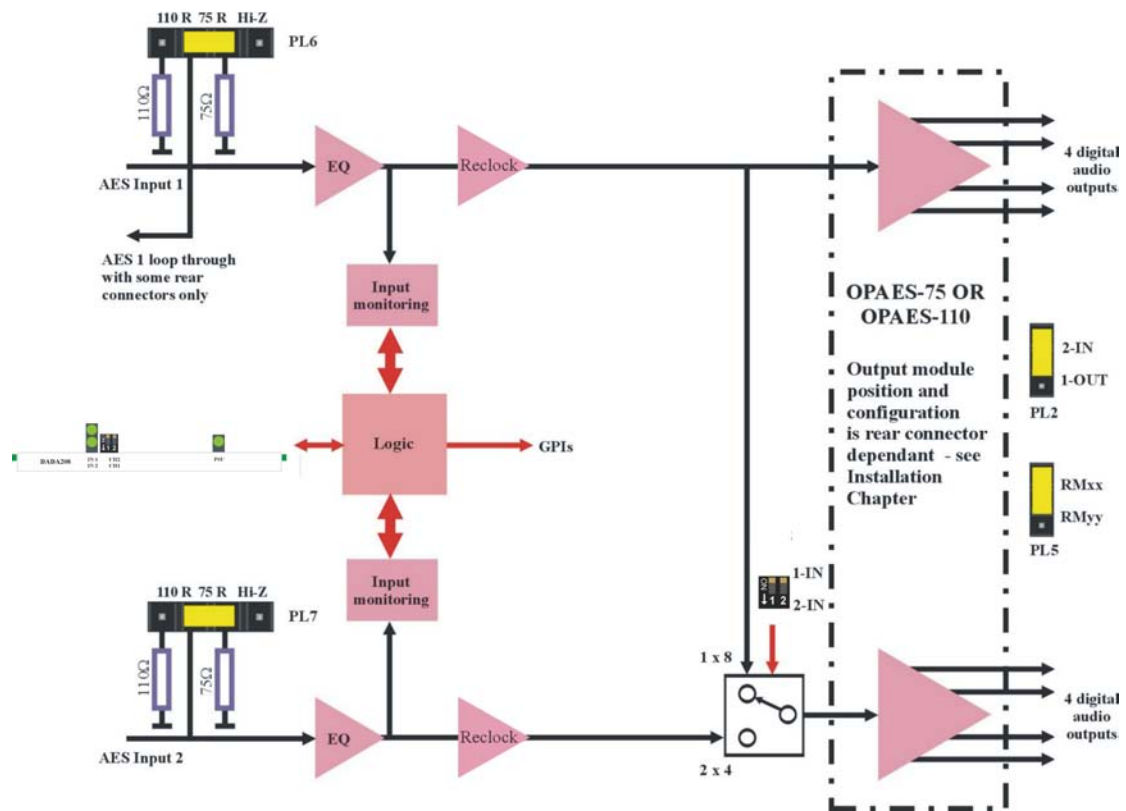
DADA208 reclocked dual digital audio DA
