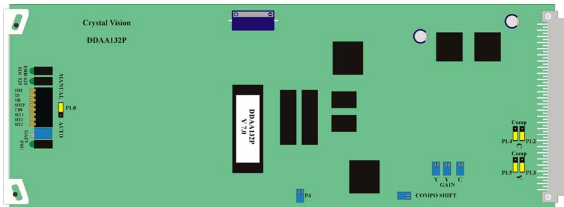
DDAA132P showing configuration jumpers
