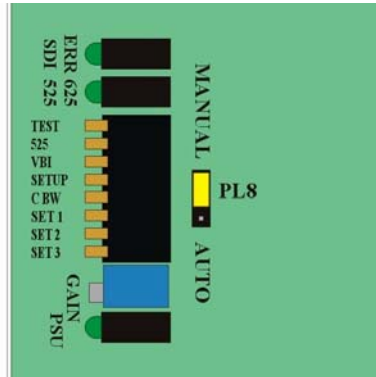
DDAA132P showing configuration jumpers
