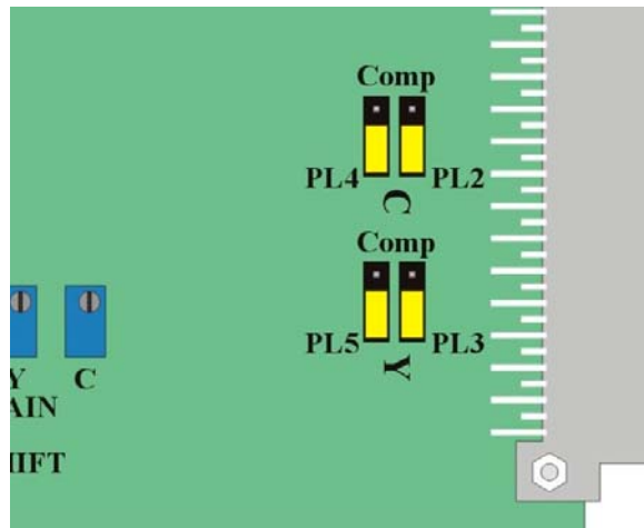
DDAA132P showing configuration jumpers
