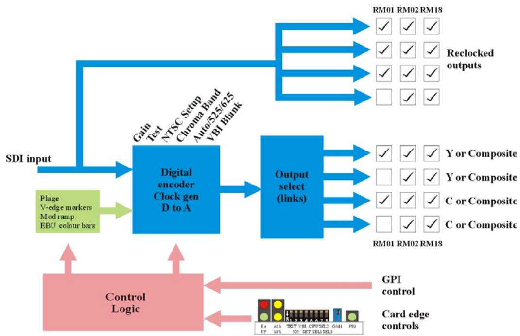
DDAA132P serial digital to analogue converter
