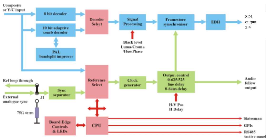
The DEC104S analogue composite or Y/C to serial digital video decoder
