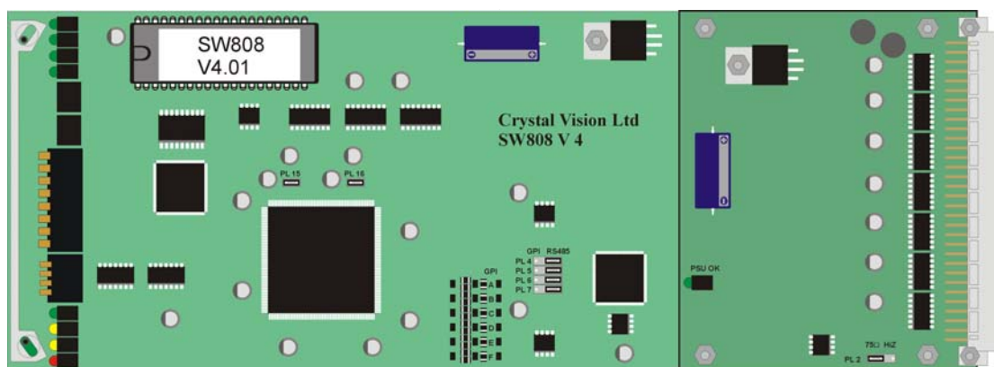
SW808 showing configuration jumper links
