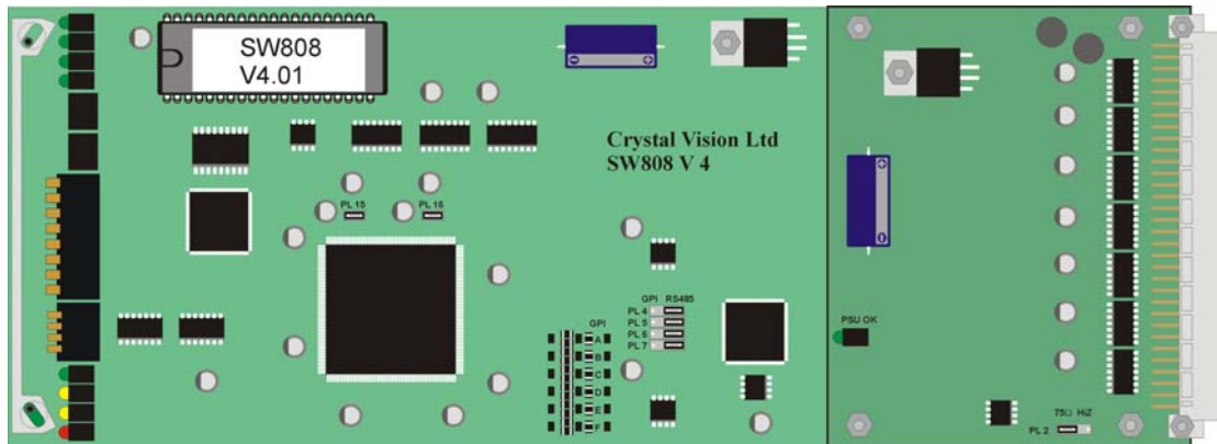
Change the six resistors marked A, B, C, D, E, F to 0Ω 0805 type for external 5 - 24V bulbs
