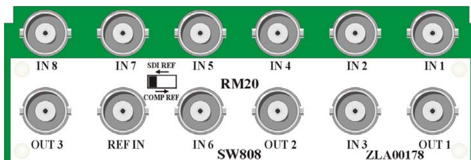
RM20 showing reference select switch
