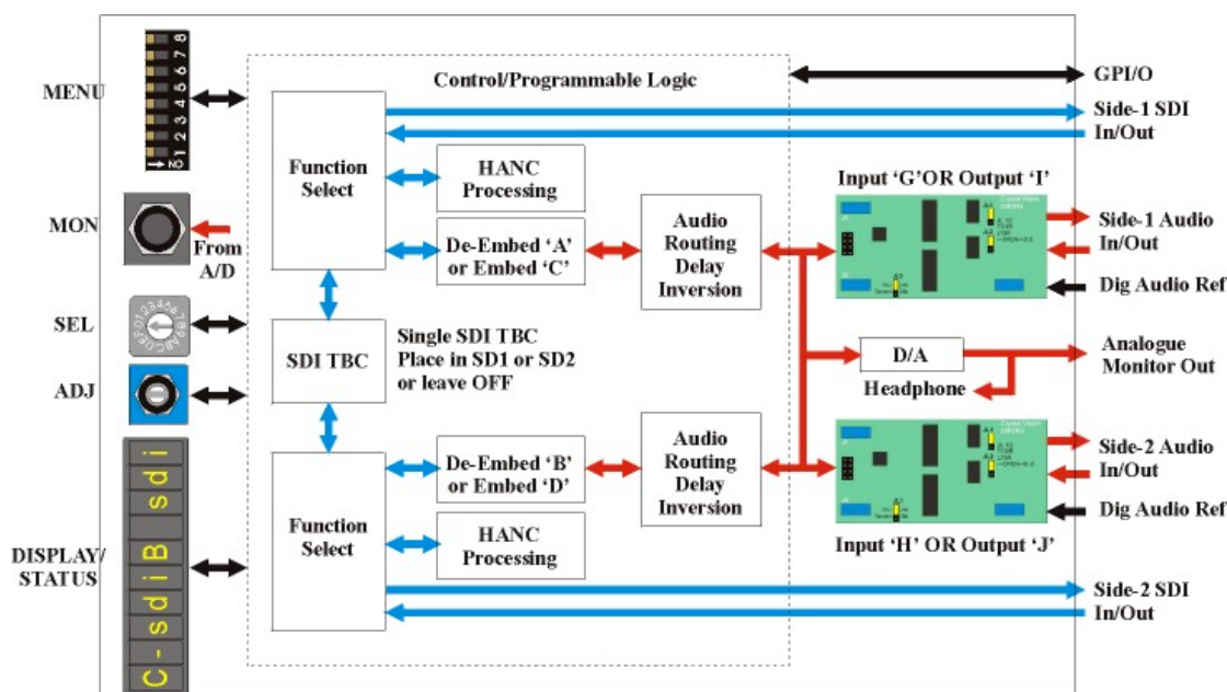
Tandem-100 architecture
