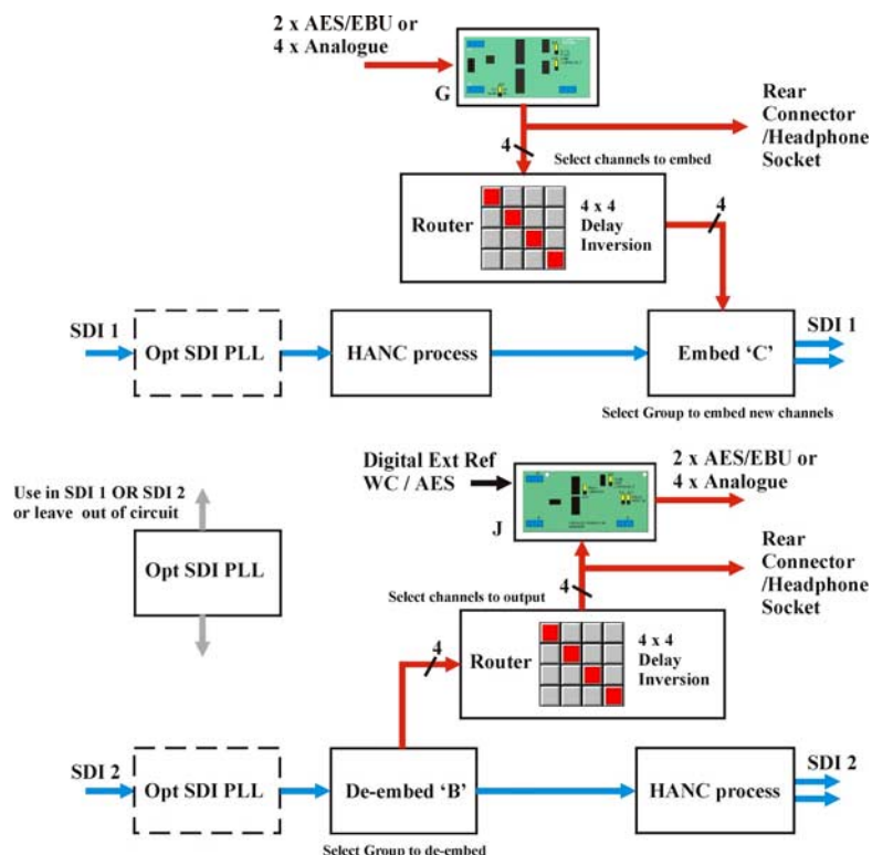
Tandem-100 with input opt side 1/output opt side 2 - option card assignment must be as shown for mixed embedder/de-embedder
