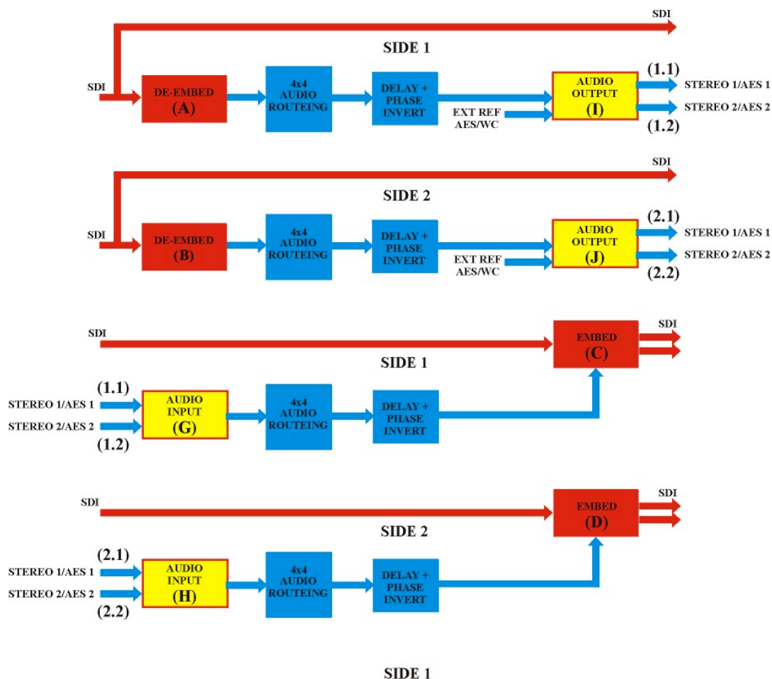
Tandem-100 modes with card edge codes
