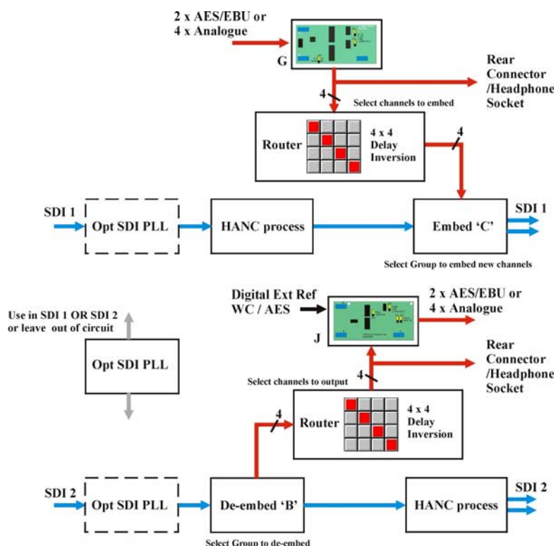
Tandem-100 as mixed embedder
