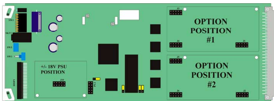
Tandem-100 - option card positions #1 and #2
