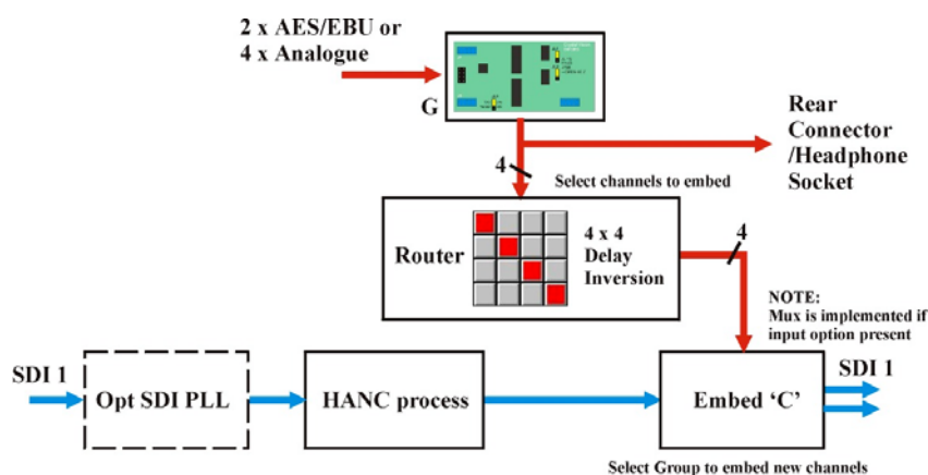
Tandem-100 side 1 with input option
