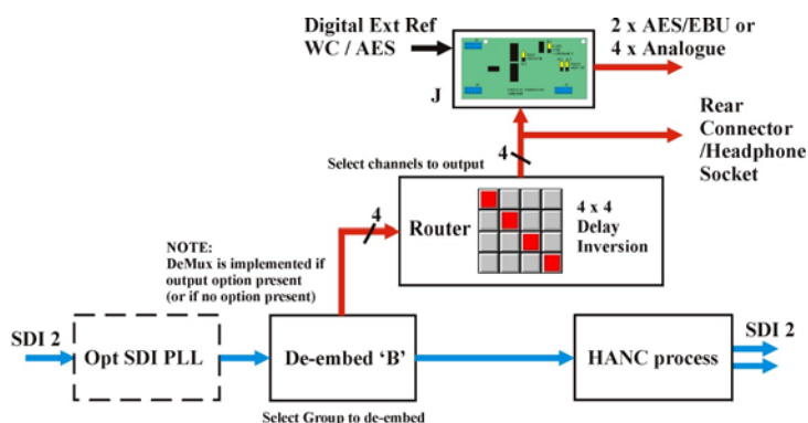
Tandem-100 side 2 with output option
