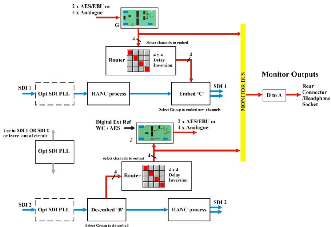
Tandem-100 audio monitoring
